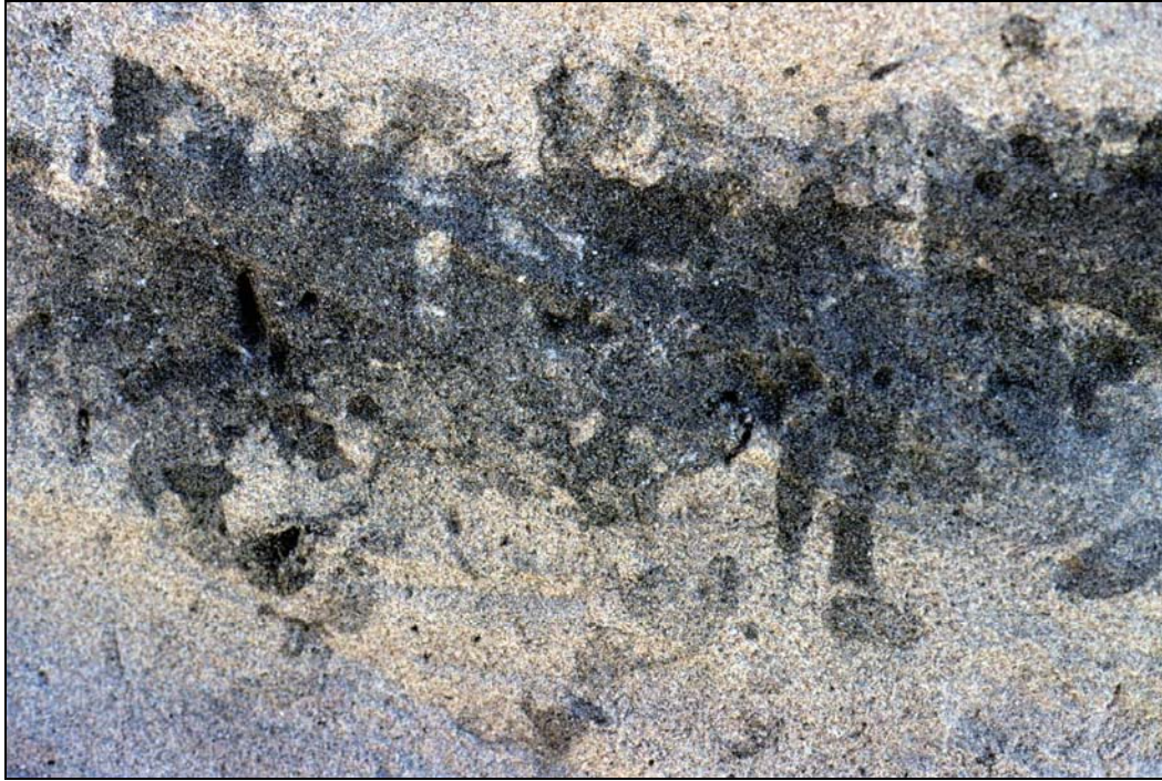
Cicada insect burrow fills, thin charcoal zone associated with a hearth, Rio del Oso alluvium, radiocarbon dated 3110 \pm 60 ^{14}\text{C} years BP (S. A. Hall and R. D. Periman, 2007, Unusual Holocene alluvial record from Rio del Oso, Jemez Mountains, New Mexico: Paleoclimatic and archaeological significance: New Mexico Geological Society Guidebook, 58 th Field Conference, Geology of the Jemez Mountains Region II , p. 459-468).
